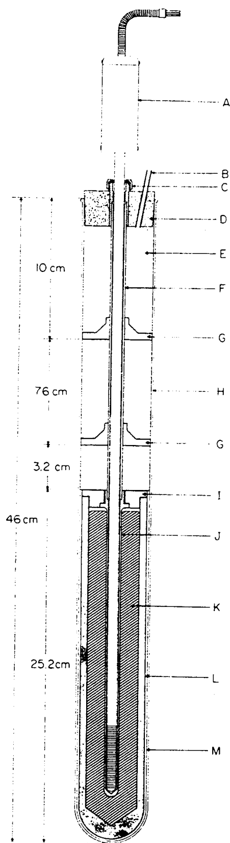
Figure 1. A schematic of a tin freezing-point cell [2] showing: (A) a 25.5 \Omega SPRT; (B) fill tube to inert gas (Ar or He) supply and pressure gauge; (C) thermometer gas seal (a modified Swagelok fitting with a silicone-rubber O-ring); (D) silicone rubber stopper; (E) thermal insulation (1.2 cm thick washed Fiberfrax disks); (F) matte-finished borosilicate-glass guide tube; (G) two graphite heat shunts; (H) precision-bore borosilicate-glass envelope; (I) graphite cap; (J) graphite re-entrant well; (K) metal sample; (L) graphite crucible; (M) thermal insulation between the borosilicate-glass envelope and the graphite crucible.
