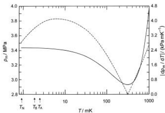
Figure : The ^3\text{He} melting pressure p (full line) and the absolute value of the derivative dp/dT (dashed line) vs. temperature. T_N , T_B and T_A indicate the temperatures of three phase transitions in solid or liquid ^3\text{He} .
